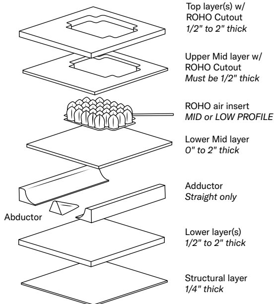
LOW PROFILE® insert (2.25" cell height, 12.5" wide, 9" deep) (CD-ROHO-LOW)
